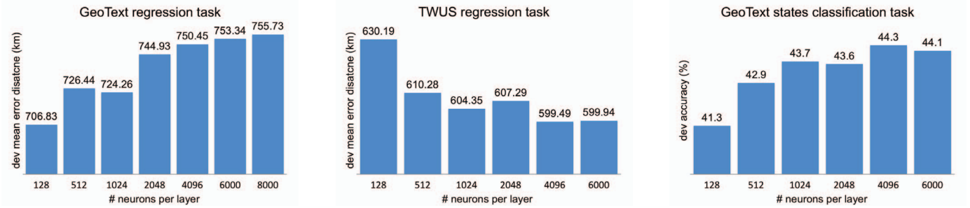
Figure 3: Varying number of neurons per layer
