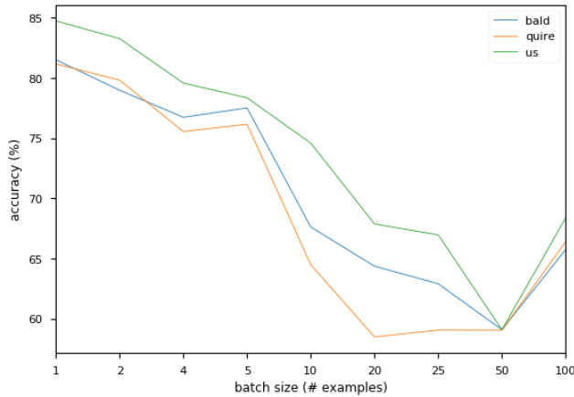
Figure 4: A view of performance of the CNNcontext model trained under different active learning methods. This is a look at the performance after 100 examples have been scored. As can be seen, compared to the fully sequential approach of one example at a time, there is approximately only 5% decrease in the performance of using a slightly larger batch size of 5 examples.
