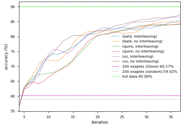
Figure 5: Comparison of interleaving and classic training sessions in terms of accuracy.
